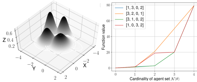
Fig. 2. True observation models p_{z_i}(z_{i,t}|\theta) = N(\mathbf{x}_i - \theta, \|\mathbf{x}_i - \theta\|I_2) . for 4 agents (left) and diversity function values F(\mathcal{G}) with varying number of set elements (right).
