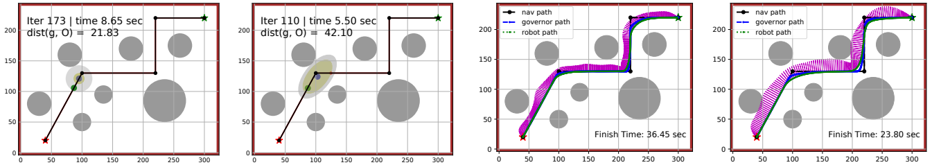
Fig. 6: Simulation of the robot-governor system tracking a piecewise-linear path (black) in an environment with circular obstacles (dark gray circles). The start and end of the path are indicated by a red and green star, respectively. The two plots on the left show that the robot at around the same location behaves differently due to different distance measures. The controller using Euclidean distance is overly cautious with respect to lateral obstacles resulting in conservative motion. The system employing SDDM trajectory bounds has a larger local safe zone, which helps the robot turn fast and smoothly. The two plots on the right show the trajectories followed by the systems employing the two controllers. The velocity profiles are shown as magenta arrows perpendicular to the robot path. The controller based on SDDM trajectory bounds (rightmost) results in higher velocities compared to the controller using Euclidean ball invariant sets. Note that the path followed by the robot (green line) is also smoother, especially when turning, for the directional controller despite the higher velocity.
