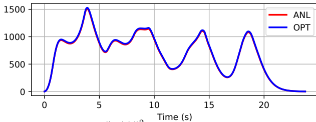
Fig. 7: Output peak \|\mathbf{x}(t)\|_{\mathbf{Q}(t)}^2 from the trajectory followed in Fig. 6. The red curve is \eta(t, \mathbf{Q}(t)) obtained analytically from eq. (6). The blue curve is \delta(t) computed from the SDP optimization in eq. (9). It is clear that \delta(t) is an upper bound for \eta(t, \mathbf{Q}(t)) , and the bound is tight at certain moments. Analytical bounds are used in simulation, while optimization bounds are computed for comparison purpose.
